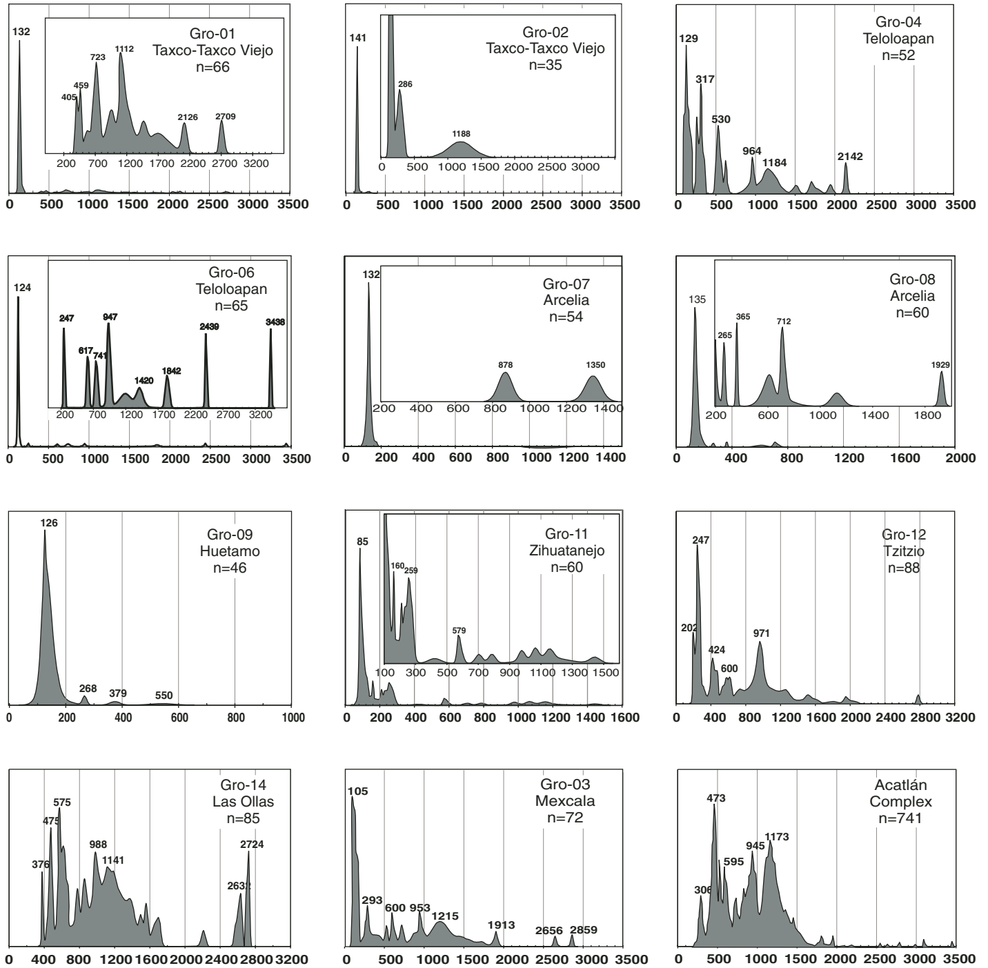
Figure 6. Cumulative-age plots of volcano-sedimentary successions of the southern Guerrero composite and western Mixteca terranes. Vertical axis is relative age probability.
