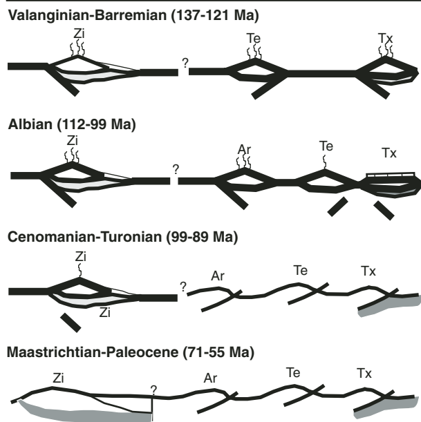
Figure 7. Paleogeography of western Mexico during Early Cretaceous time and tectonic evolution of the Guerrero and western Mixteca arc successions. NA—North America; Ne—Nevada; Kl—Klamaths; Al—Alisitos; Tx—Taxco-Taxco Viejo; Te—Teloapan; Ar—Arcelia; Zi—Zihuatanejo; Ac—Acatlán; Ox—Oaxaca; Ch—Chortis block; PCA—proto-Caribbean arc. Gray pattern indicates crustal substratum.
