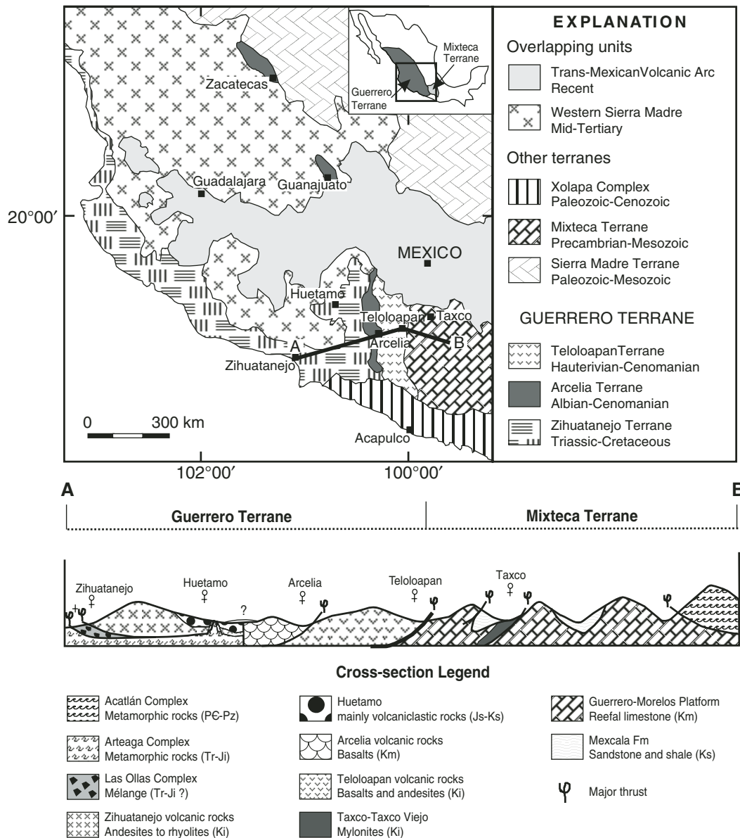
Figure 1. Terrane map of southwestern Mexico and schematic cross section showing distribution and structural relationship of Upper Jurassic–Cretaceous volcanic arc successions of southern Guerrero and western Mixteca terranes (after Mendoza and Guerrero, 2000).
