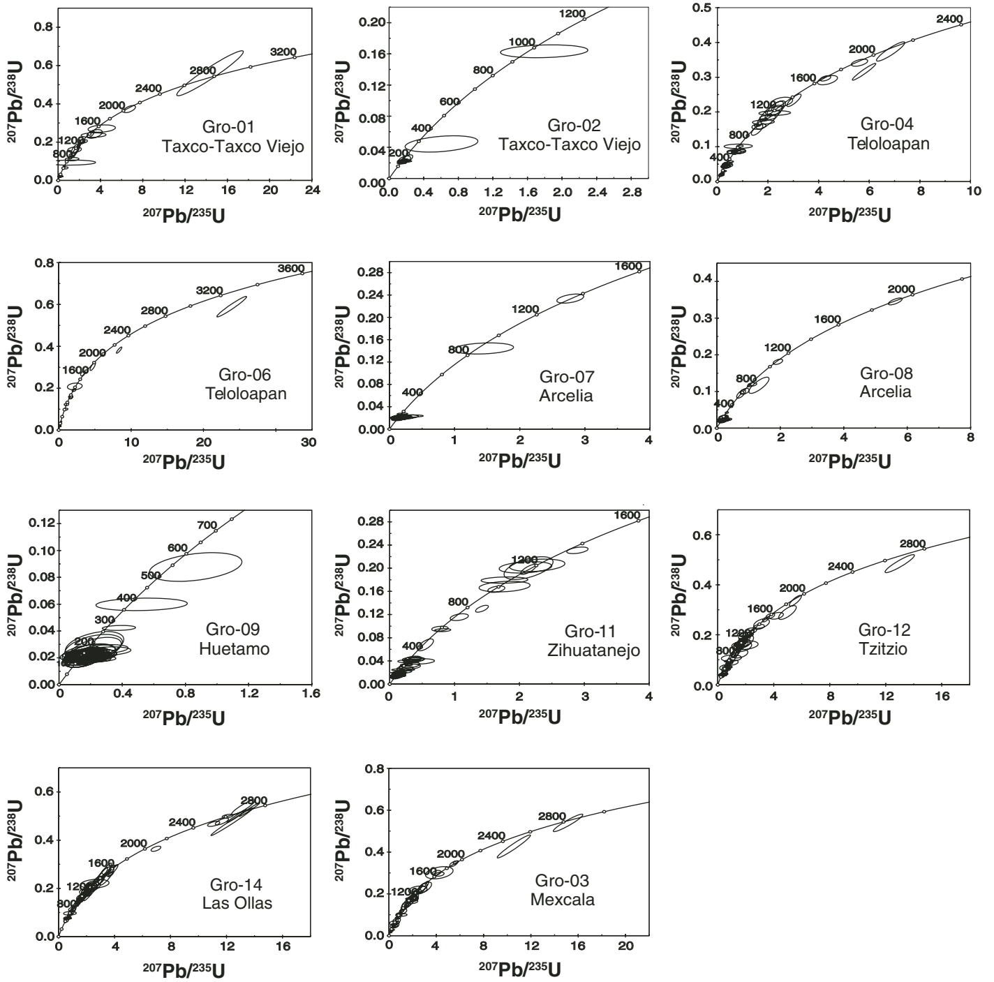
Figure 5. Concordia diagram showing U/Pb age data of detrital zircons from volcano-sedimentary sequences of the southern Guerrero composite and western Mixteca terranes. Ellipses are 1 \sigma sigma.
