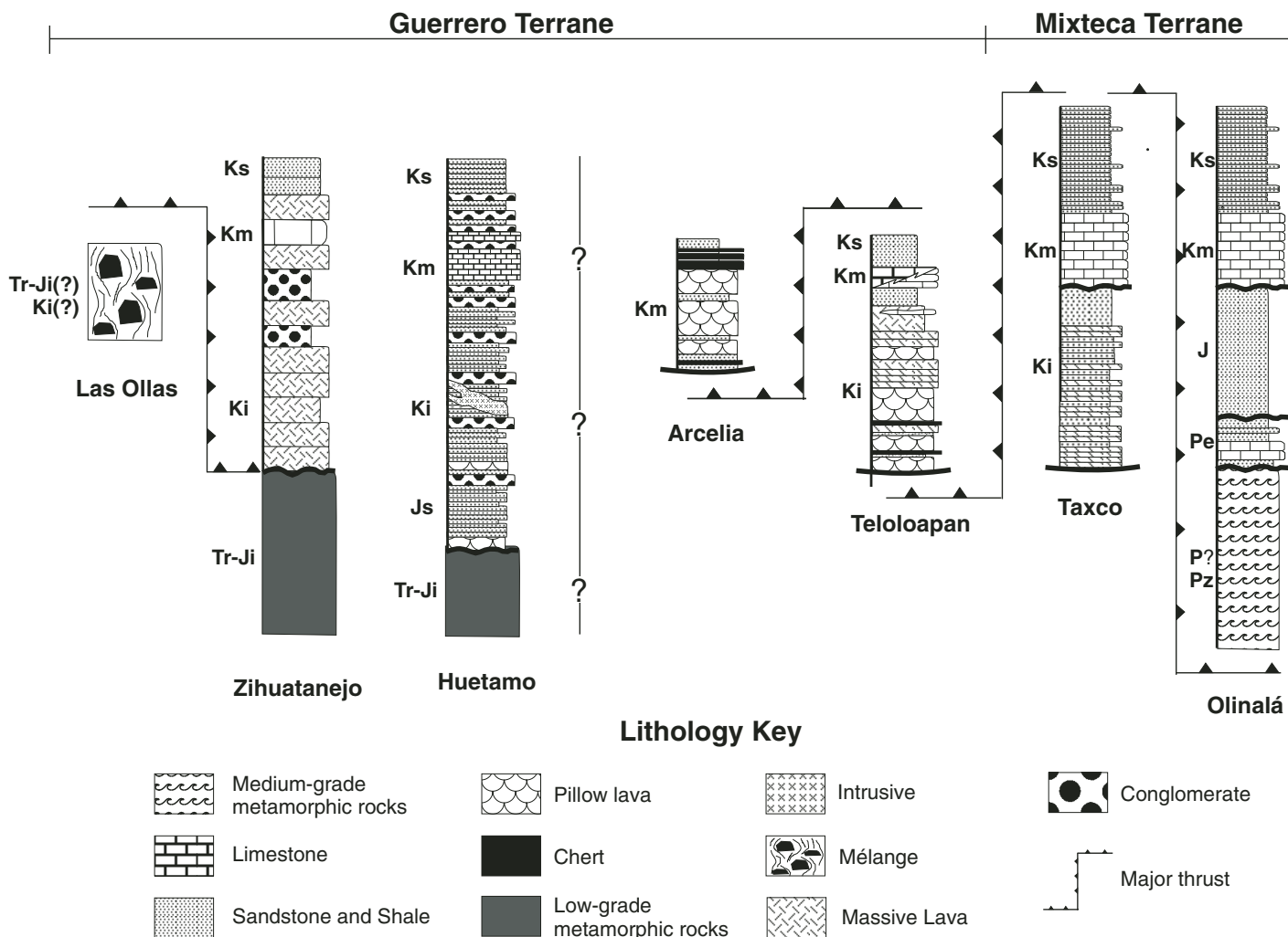
Figure 3. Stratigraphy and structural relationship of studied successions (after Talavera, 1994).
