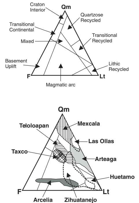
Figure 4. Ternary diagram illustrating the composition of sandstone from the southern Guerrero composite and western Mixteca terrane successions. Provenance fields are from Dickinson and Suczek (1979).
